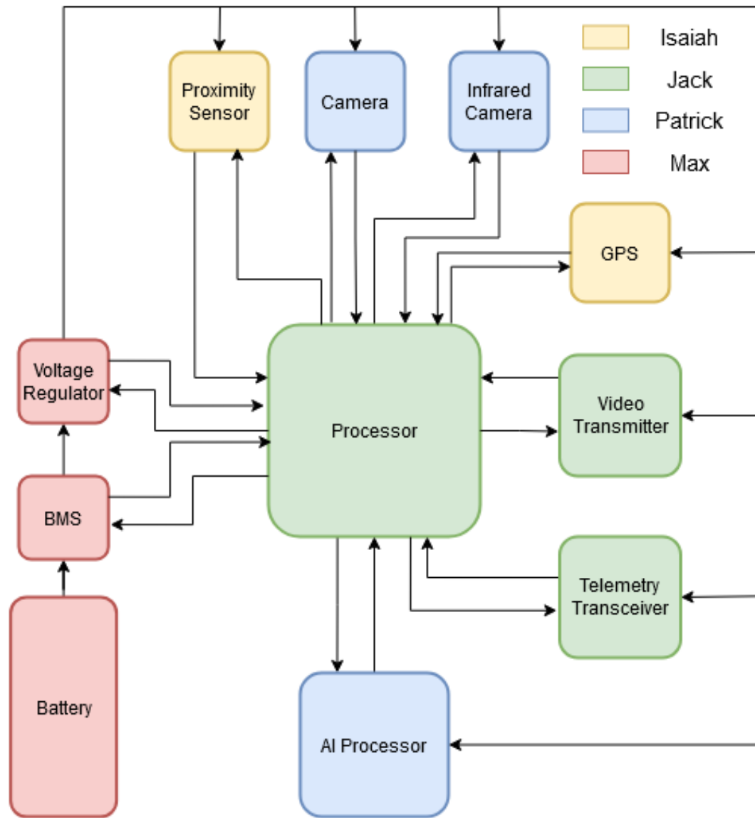
Figure 2.1. Sensor Package Hardware Block Diagram by Authors
