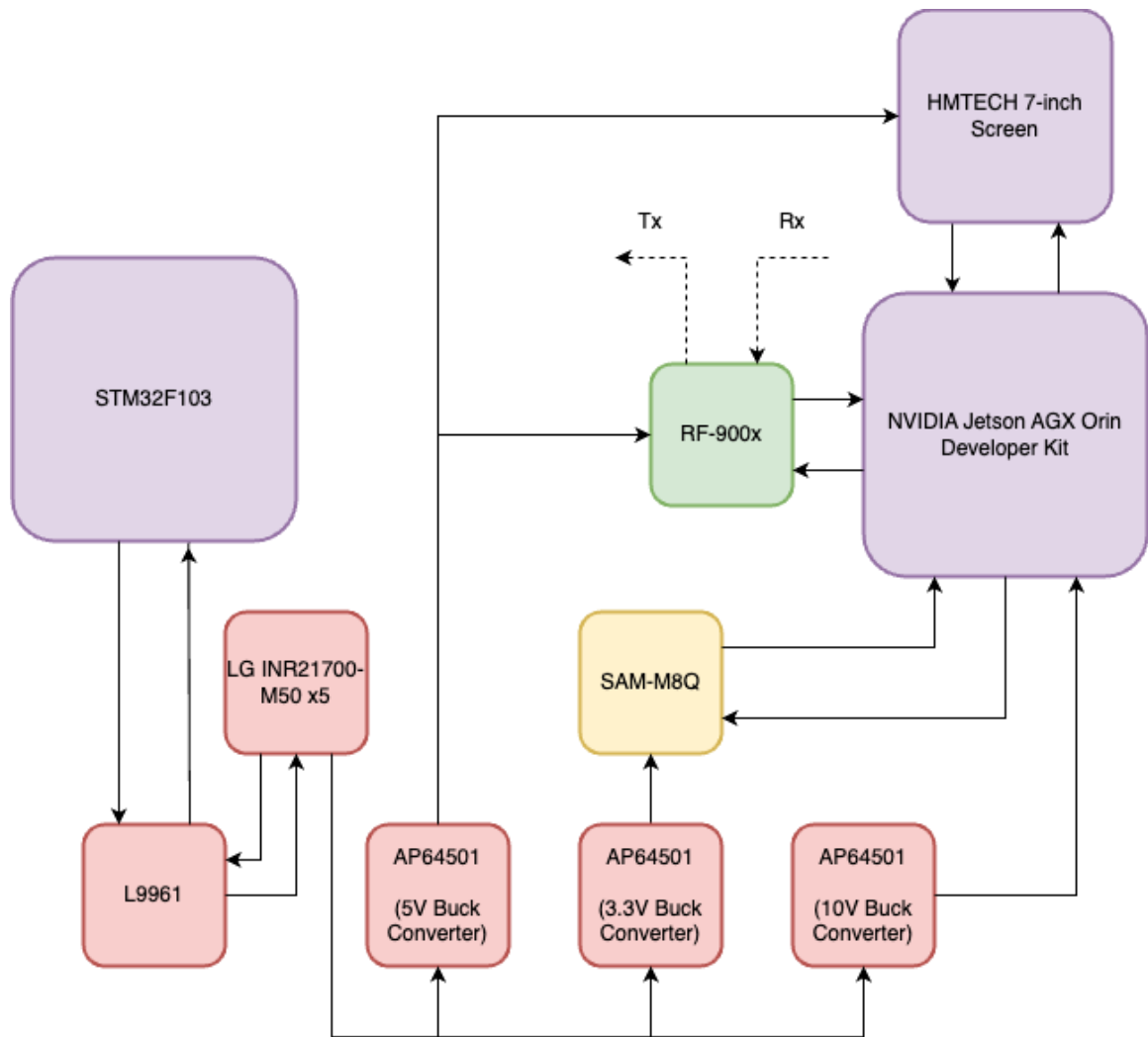
Figure 6.1. Hardware Diagram By Authors
