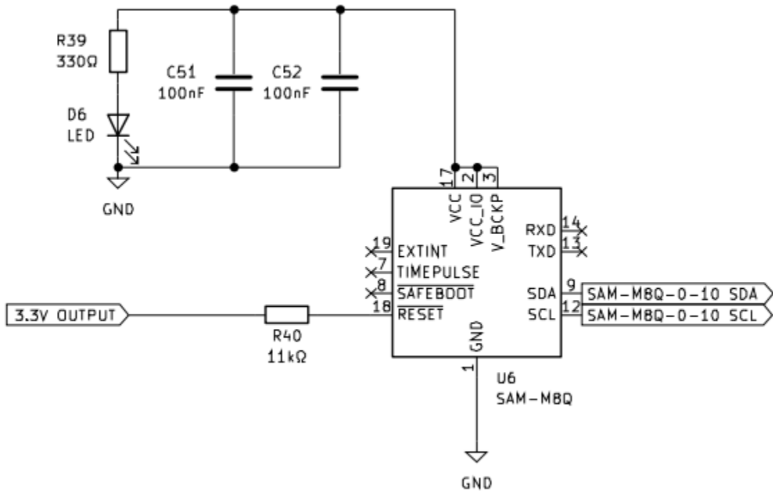
Figure 6.2. GPS Pinout By Authors
