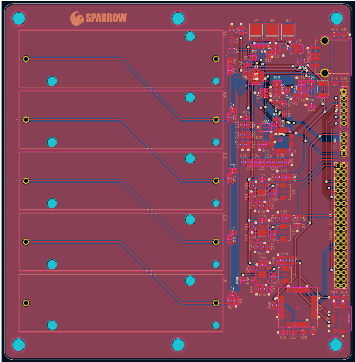
Figure 8.1. BMS Rev.1 Board Diagram by Authors
