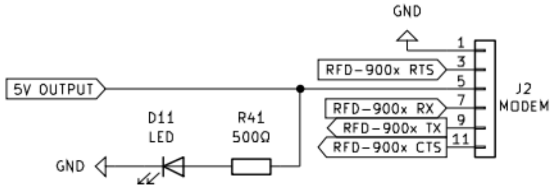
Figure 6.4. Modem Connections By Authors
