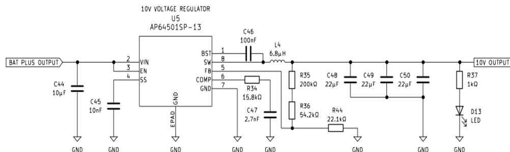
Figure 6.12. 10V Buck Voltage Regulator Schematic By Authors
