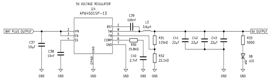
Figure 6.11. 5V Buck Voltage Regulator Schematic By Authors
