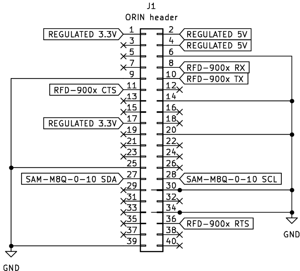
Figure 6.6. Jetson AGX Orin Developer Kit Header Connections By Authors
