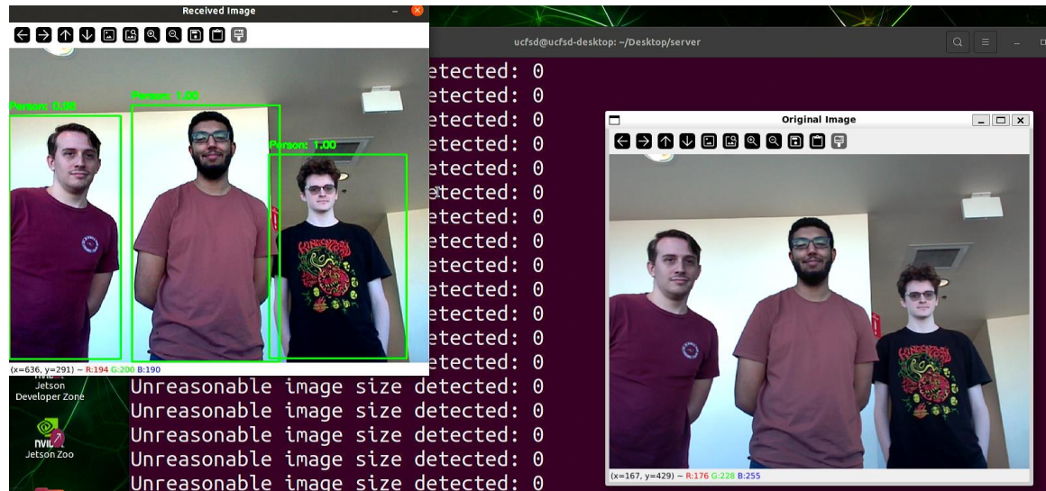
Figure 9.3. Human Detection Code Test by Authors
