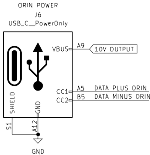
Figure 6.7. Jetson AGX Orin Developer Kit Power Connections By Authors
