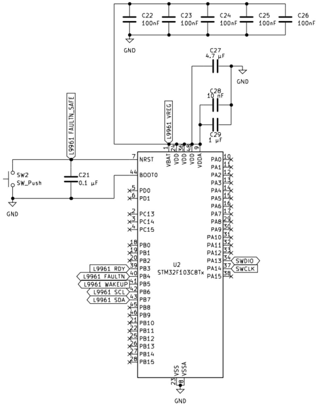
Figure 6.5. STM32F103C8T6 Pinout By Authors
