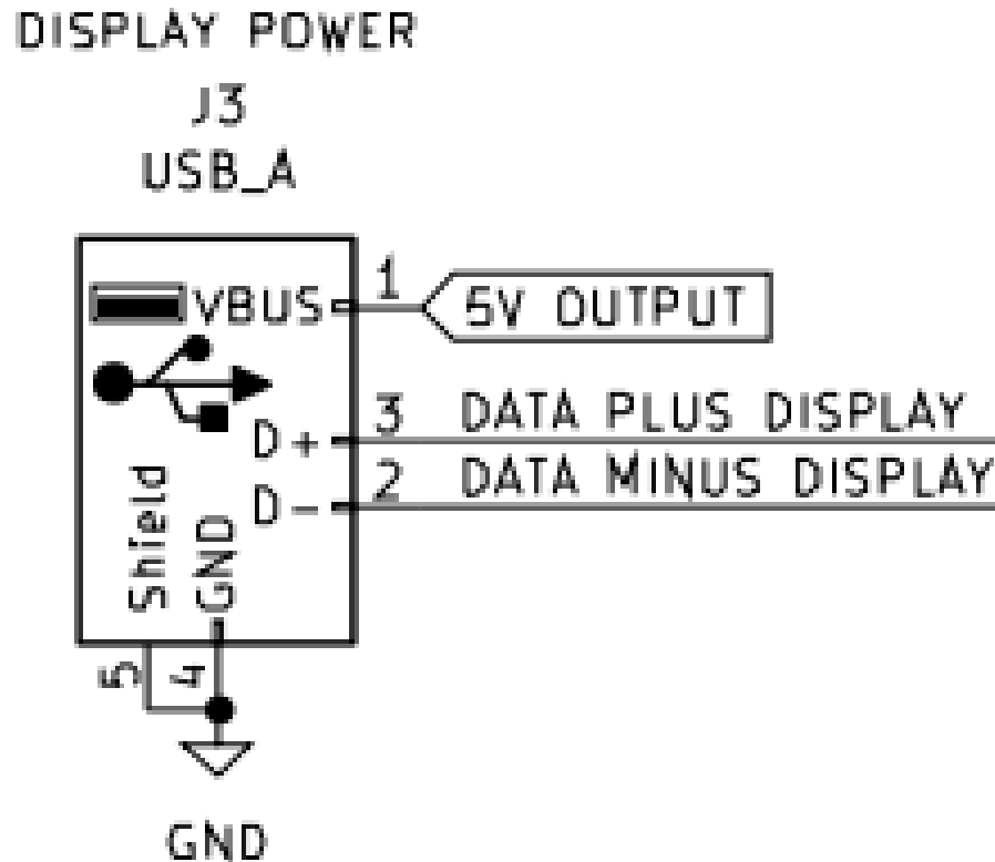
Figure 6.3. Display Connections By Authors
